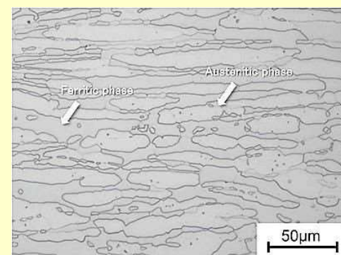
S-phase Microstructure
